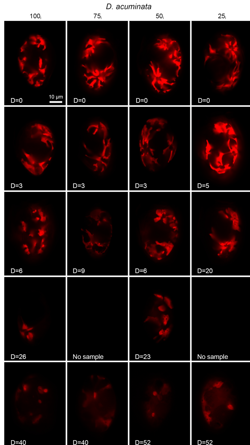
Fig 6. Epifluorescence microscopy of kleptochloroplasts in D. acuminata at the 100 i , 75 i , 50 i and 25 i incubations during the experimental period of 58–72 days. Examples of kleptochloroplasts in one cell are shown from each sampling.
